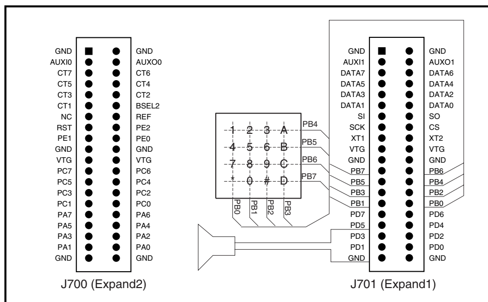
Figure 5. Schematics of the STK500 Top-Module
